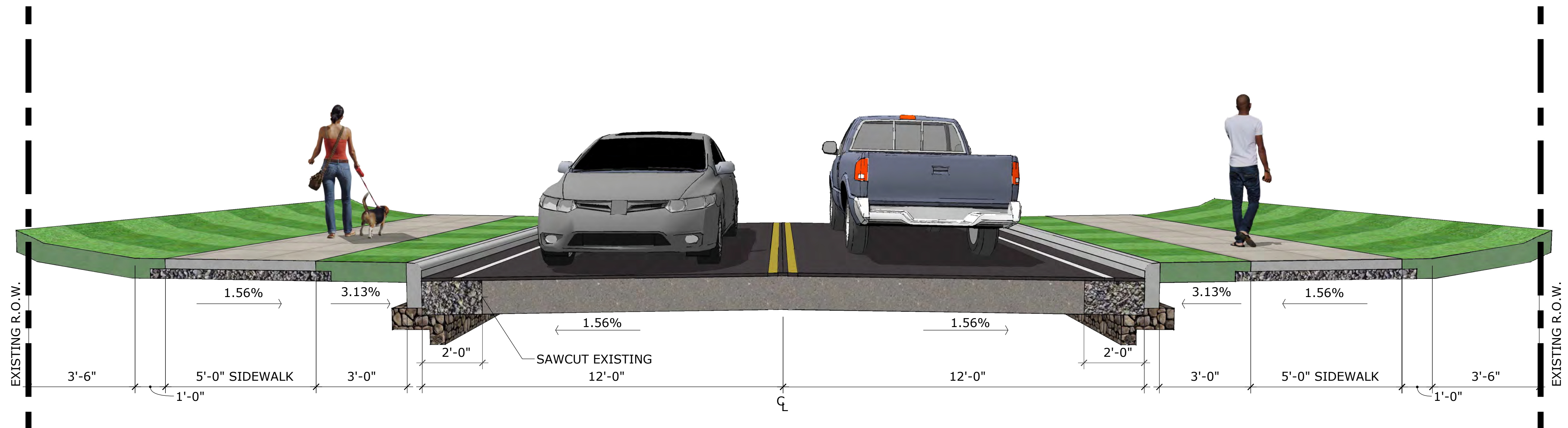
MOUND STREET - 2 LANE TYPICAL SECTION
