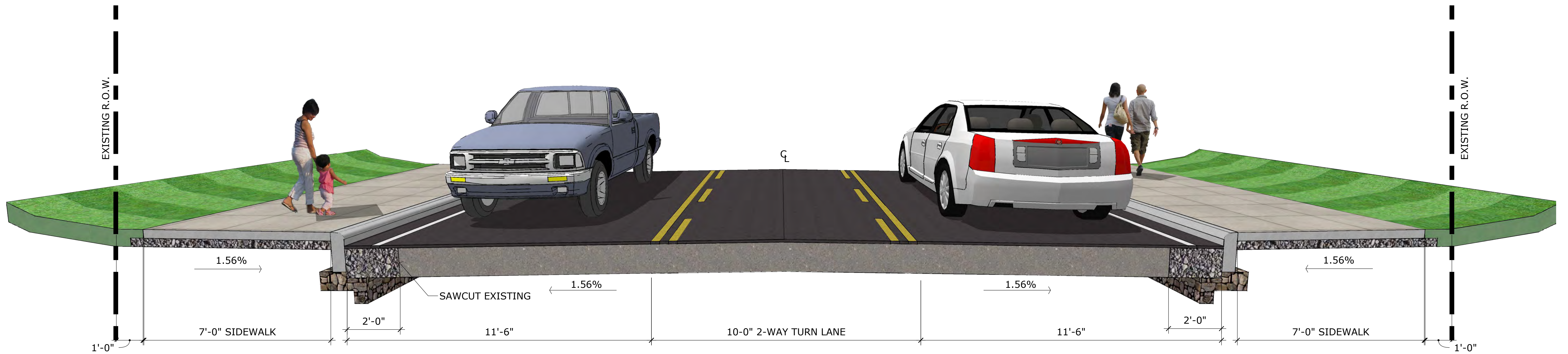
MOUND STREET - 3 LANE TYPICAL SECTION
