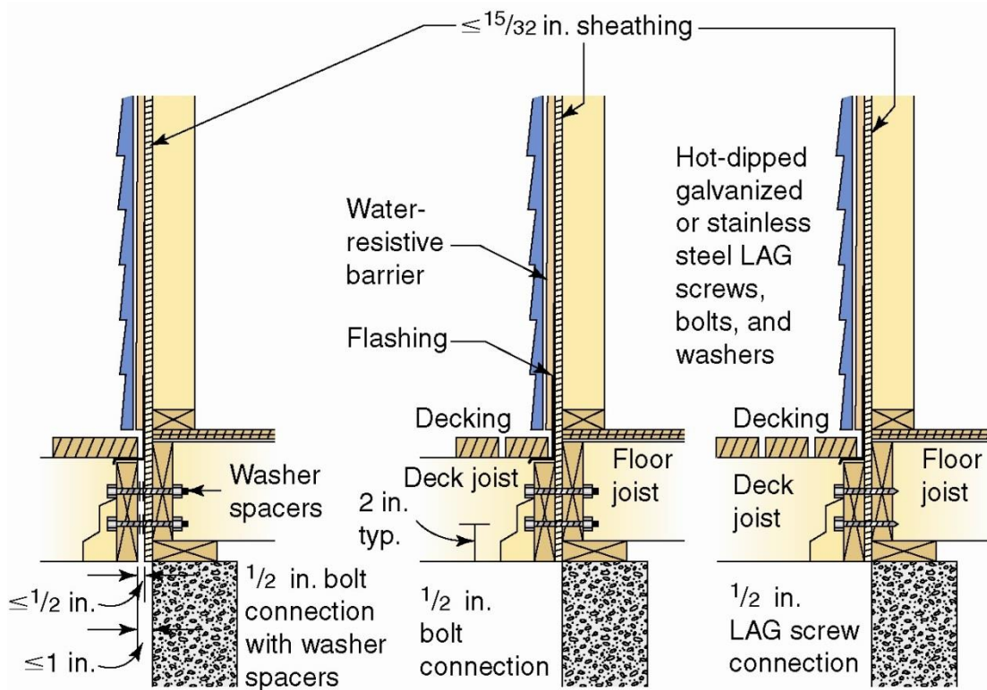
Deck ledger connection
