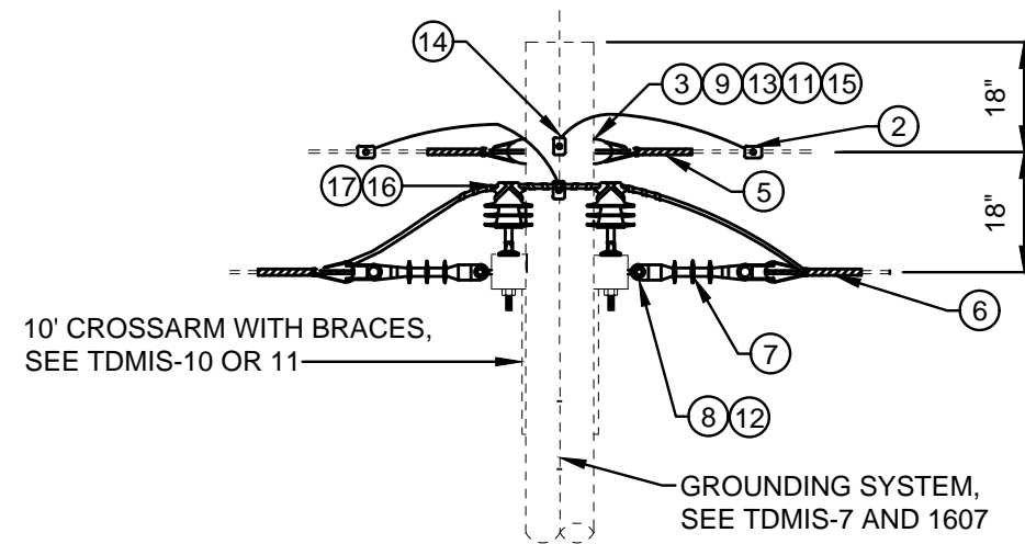
DETAIL 2 SPACER CABLE TO SPACER CABLE DOUBLE ENDED - SIDE VIEW
