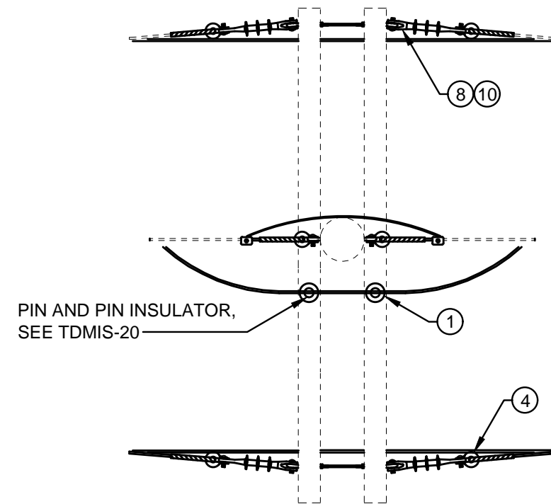
DETAIL 1 SPACER CABLE TO SPACER CABLE DOUBLE ENDED - PLAN VIEW
