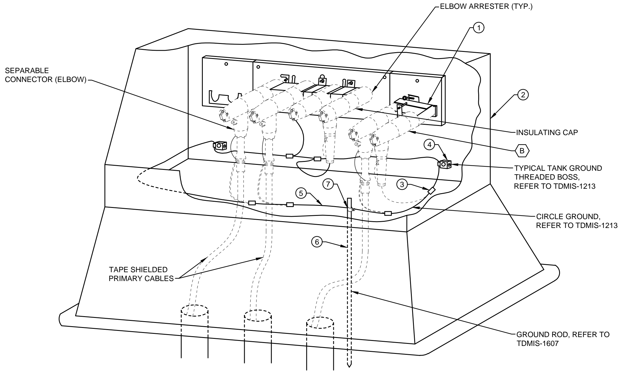
DETAIL 1 SINGLE PHASE PRIMARY ENCLOSURE 200A
