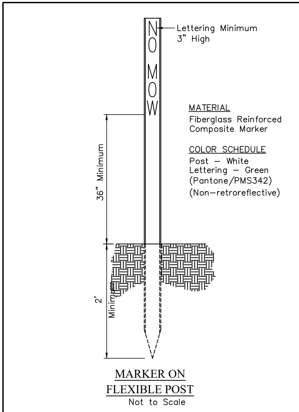
Detail Z
