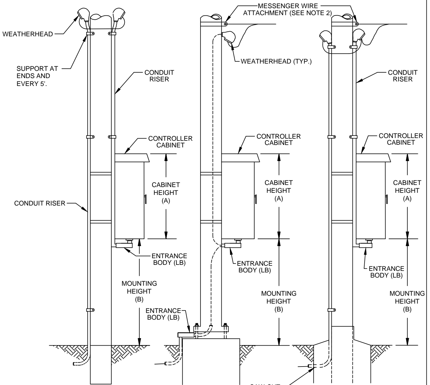
RISERS ON WOOD POLE
