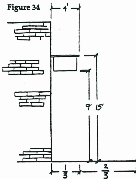
Figure 34: Projecting sign requirements.
