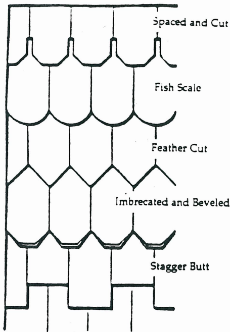
Figure 11: Types of cut wood or artificial siding shingles. Source: Cape May Guidelines.
