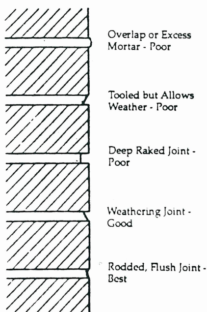
Figure 9: Types of brick joints. Source: Cape May Guidelines.
