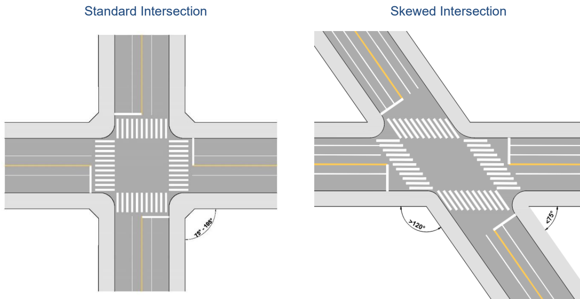
Figure 4: Intersection Skew Impact to Intersection Geometry
