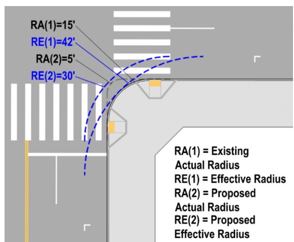
Figure 6: Example Effective and Actual Radius
