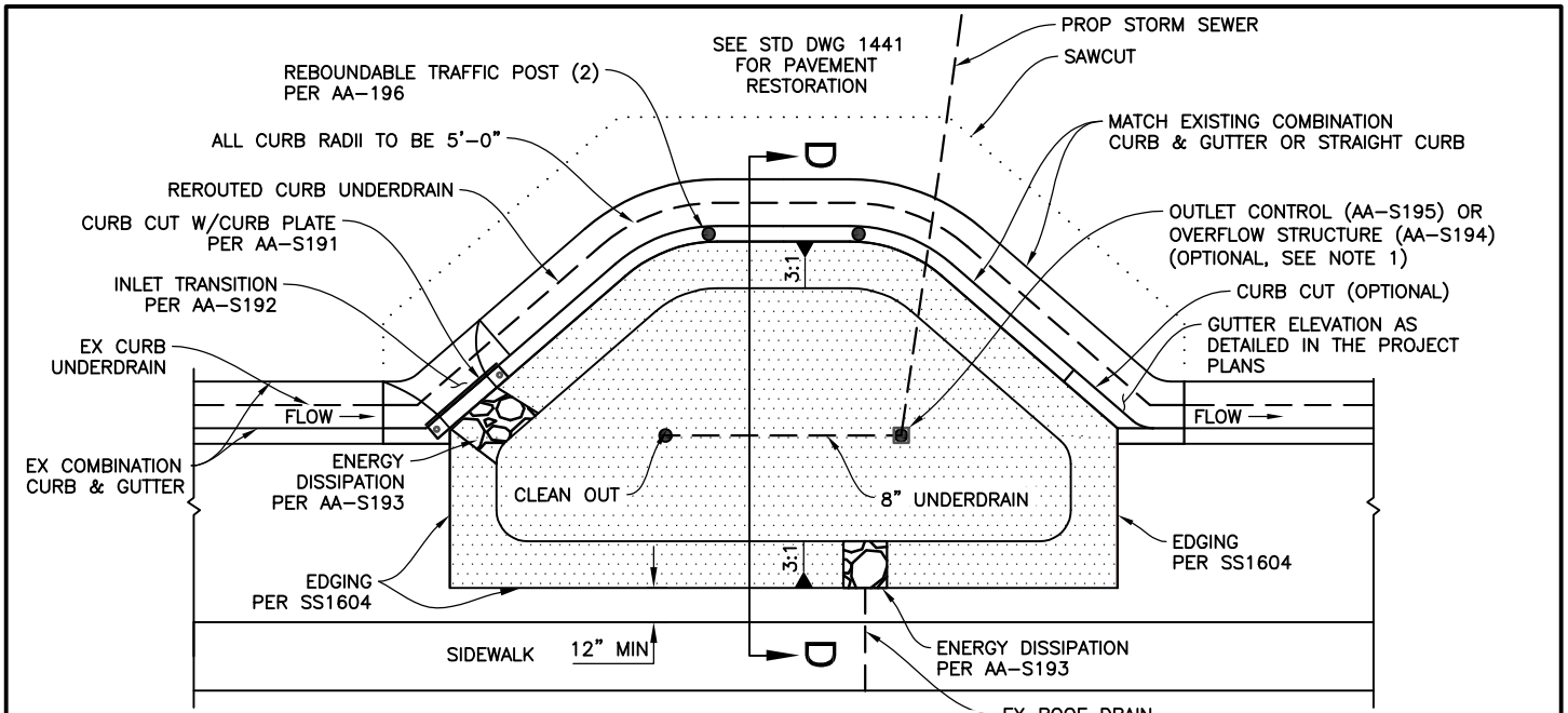
Type D Basin: Plan View
