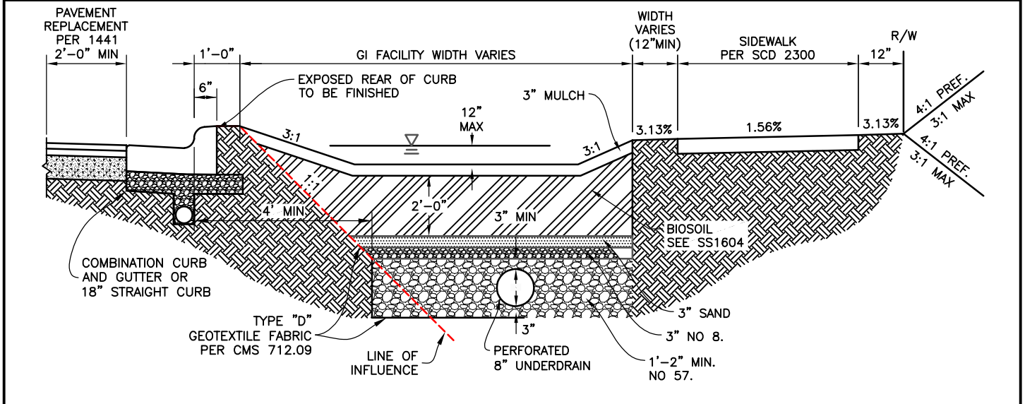
Type D Basin: Profile View
