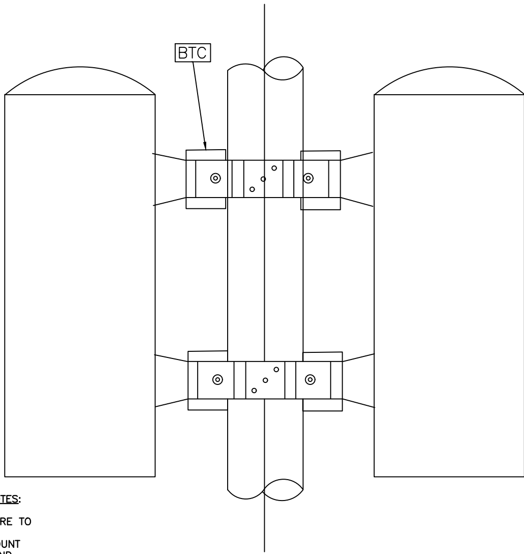
DETAIL 1 CLUSTER TYPE MOUNTING BRACKET
