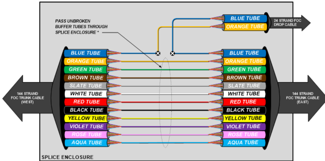
Figure 12.4 Typical Splicing Diagram – 2 cables
