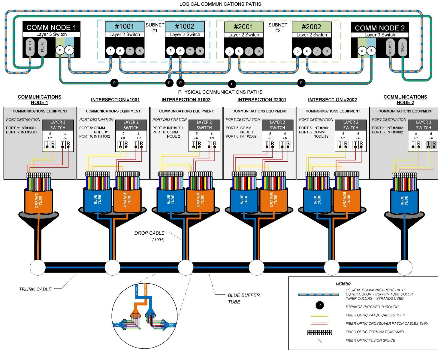
Figure 12.2 Fiber Optic Redundancy Communications Paths
