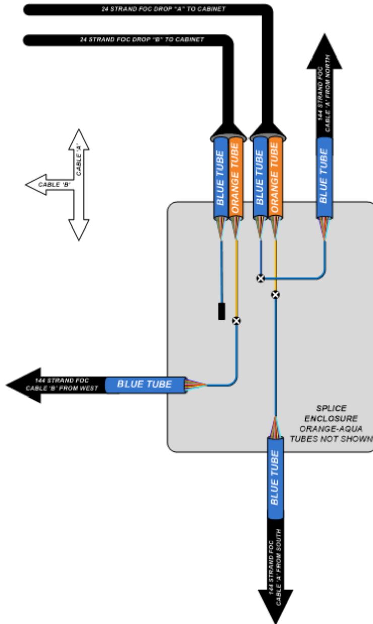
Figure 12.9 Splicing Orientation – 3 Cables
