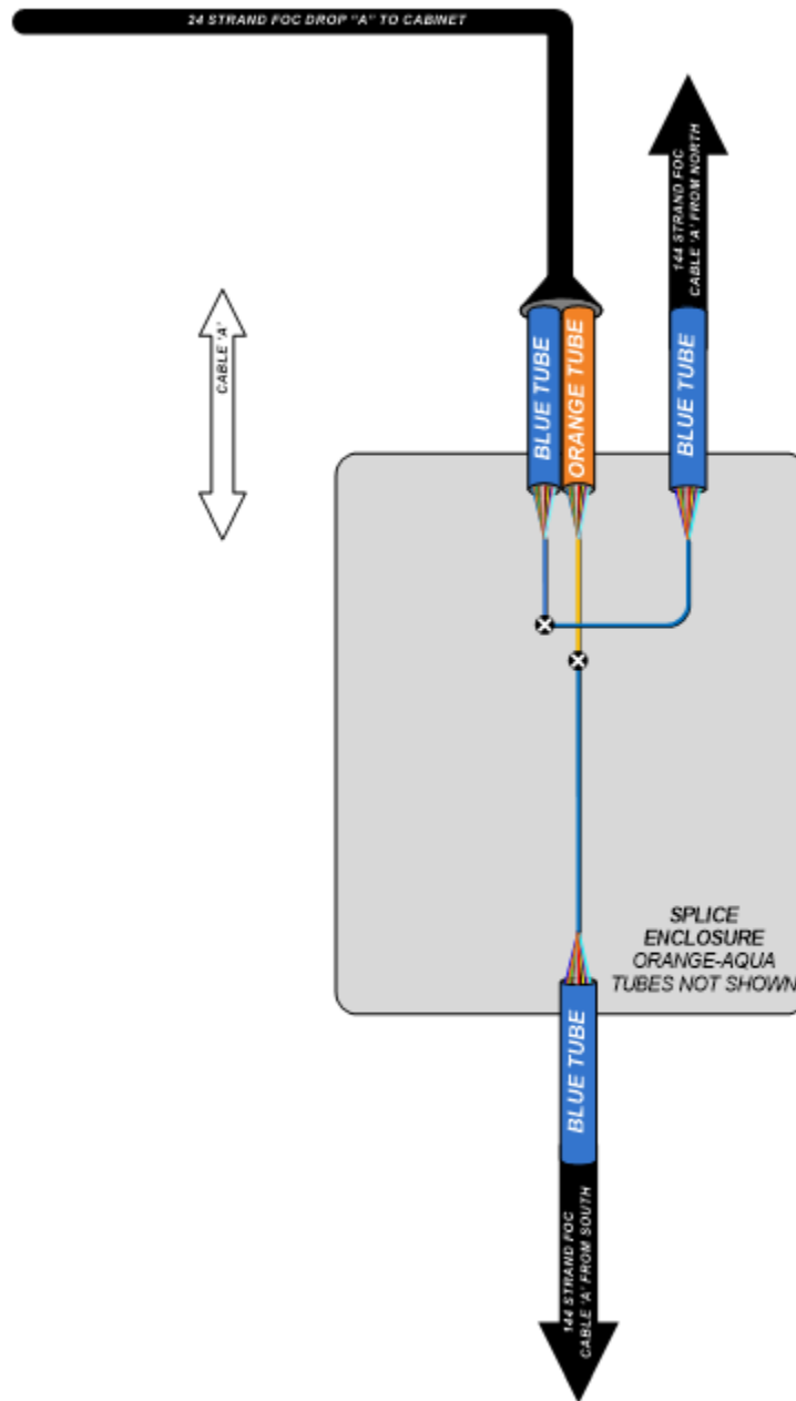
Figure 12.8 Splicing Orientation – 2 cables – North/South
