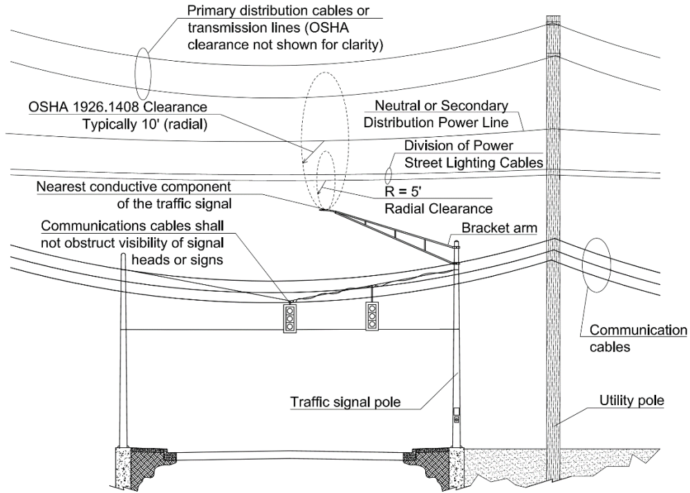
Figure 4.1 Overhead Utility Clearance Illustration (Profile View)
