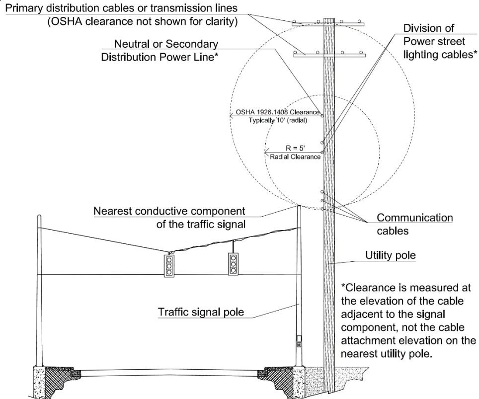
Figure 4.2 Overhead Utility Clearance Illustration (Strain Pole Cross-section View)
