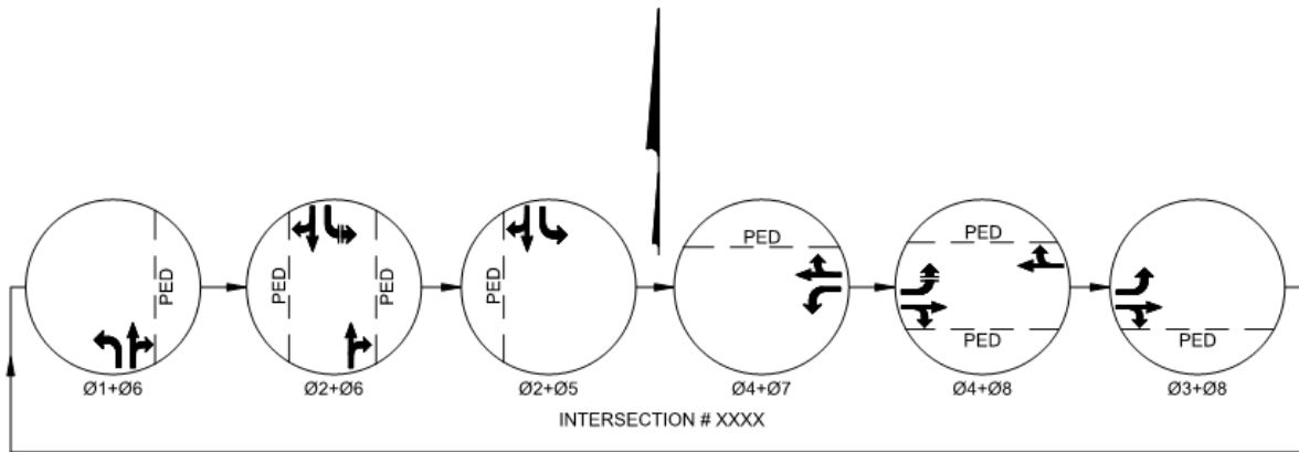
Figure 15.14 Lead-Lag Phasing Example 3 North-South Main Line
