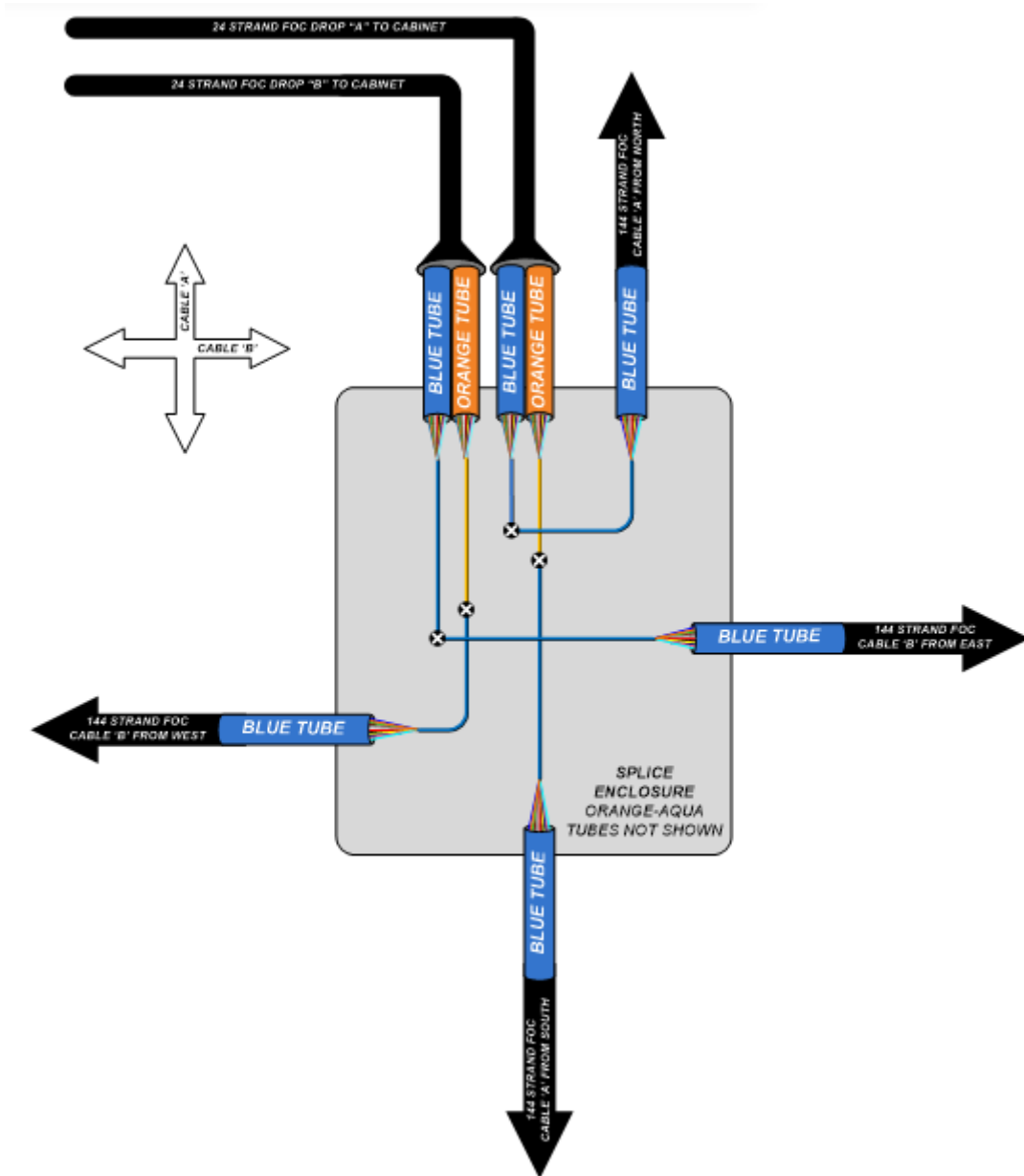
Figure 12.10 Splicing Orientation – 4 Cables
