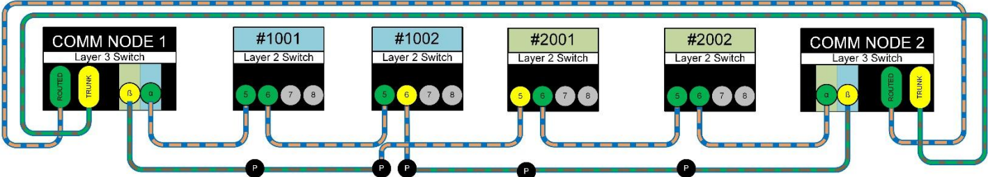
Figure 12.3 Fiber Optic Redundancy Scenarios
