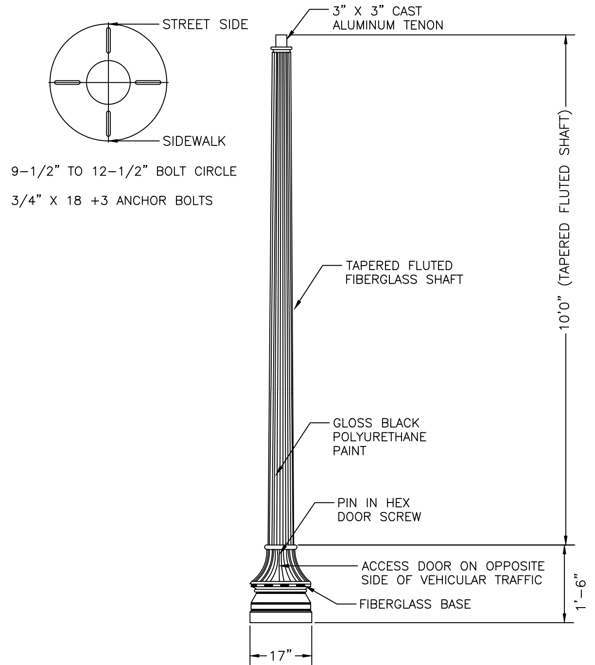
FIBERGLASS ASSEMBLY
