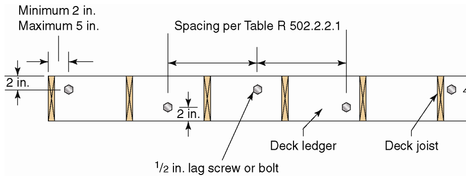
Deck ledger connection
