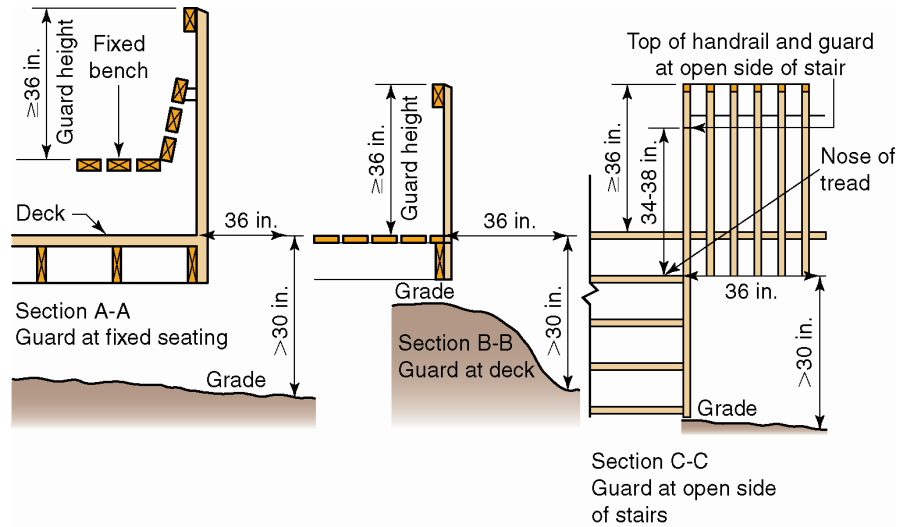
Determining required guard locations
